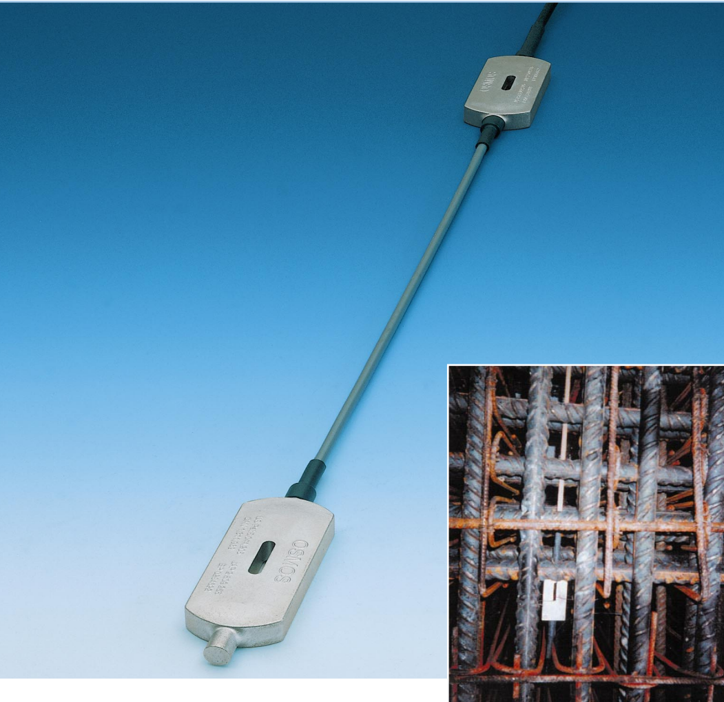
Optical Strand in a reinforcing cage.
